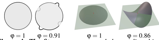
Figure 4: The fitness parameter \phi helps to disambiguate two identical fits, e.g., a smooth versus a bumped neighborhood (left), or a flat versus a saddle configuration (right).
