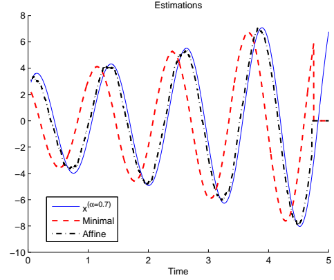
Fig. 3. \tilde{y}_{t_0}^{(0.7)}(0, 0, T) with T = 0.25 and \tilde{y}_{t_0}^{(0.7)}(0, 0, T, 0.7) with T = 0.28 .
