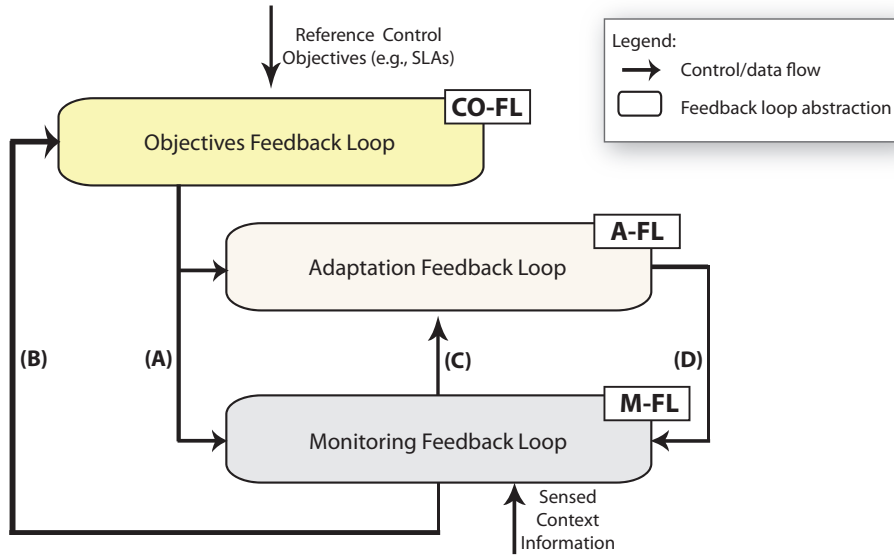
Fig. 4. The three levels of dynamics that must be controlled in context-driven self-adaptive software systems. The control objectives feedback loop, (CO-FL), controls changes in adaptation goals and monitoring requirements to ensure their fulfillment. The adaptation feedback loop, (A-FL), controls the adaptive behavior of the target system and the adaptation mechanism, according to control objectives and taking into account monitored context events. The dynamic monitoring feedback loop, (M-FL), manages context information for preserving context relevance of the adaptation mechanism. Labels (A), (B), (C) and (D) highlight the control/data flow among the feedback loops, which would require the implementation of the appropriate method interfaces.
