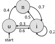
Fig. 2. Markov chain for n-grams
