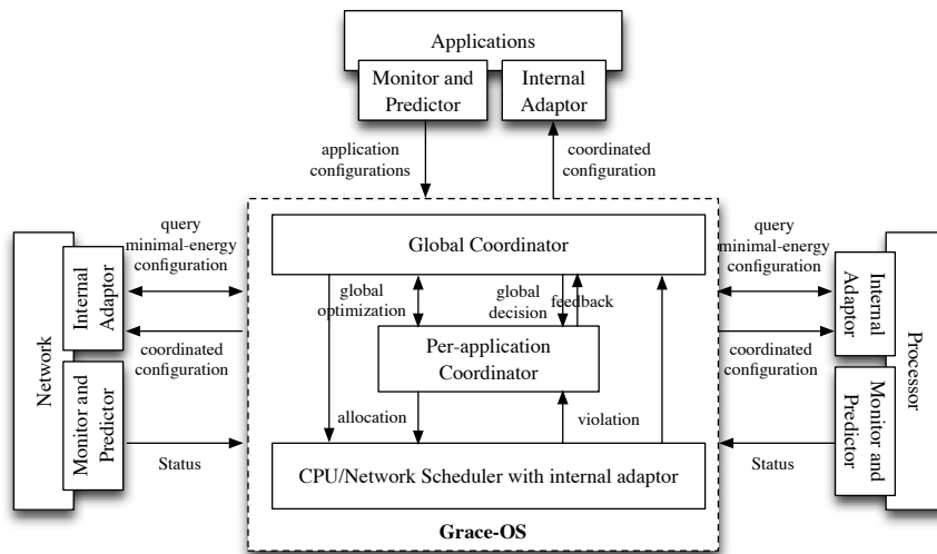
Figure 3. GRACE architecture. [6]
