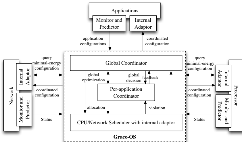
Figure 3. GRACE architecture. [6]
