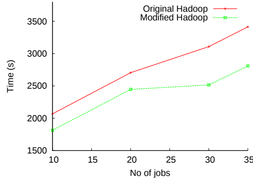
Fig. 4. Completion time for long-running pipeline applications.
