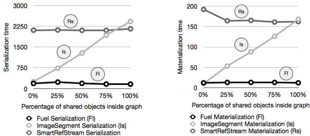
Figure 6. ImageSegment serialization and materialization in presence of shared objects.
