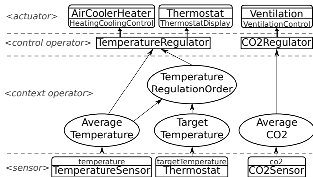
Figure 9: The HVAC system specification.
