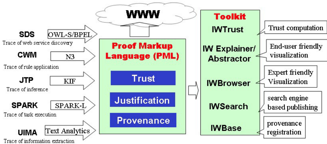
Figure 4: Inference Web Explanation Infrastructure.
