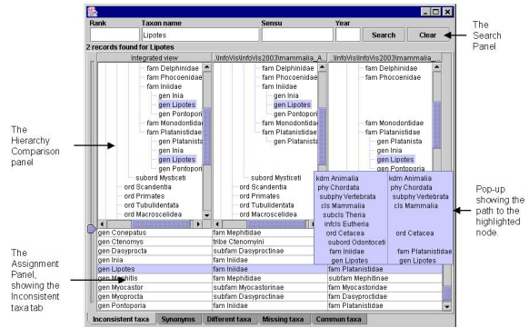
Figure 8: TaxoNote [Mor03]
