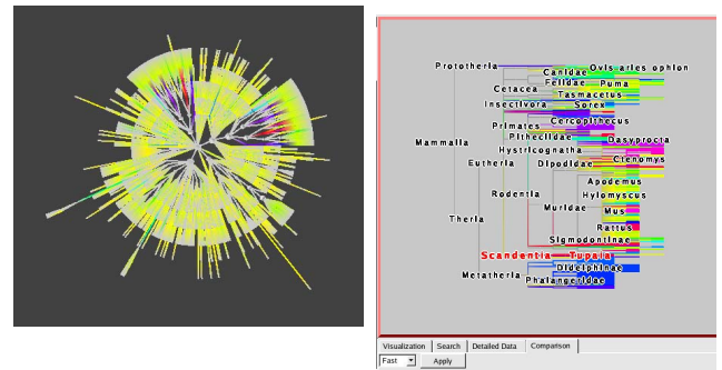
Figure 7: EVAT [Aub03]
