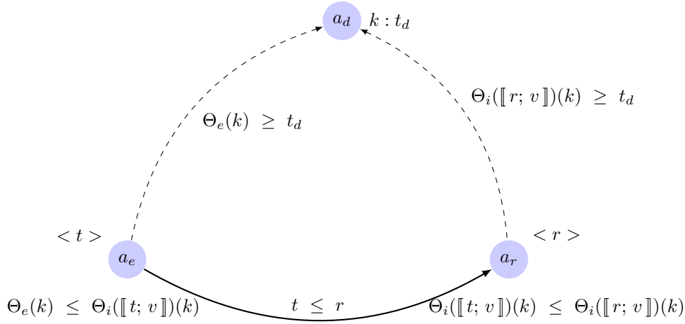
Figure 9: Communication with type inference
