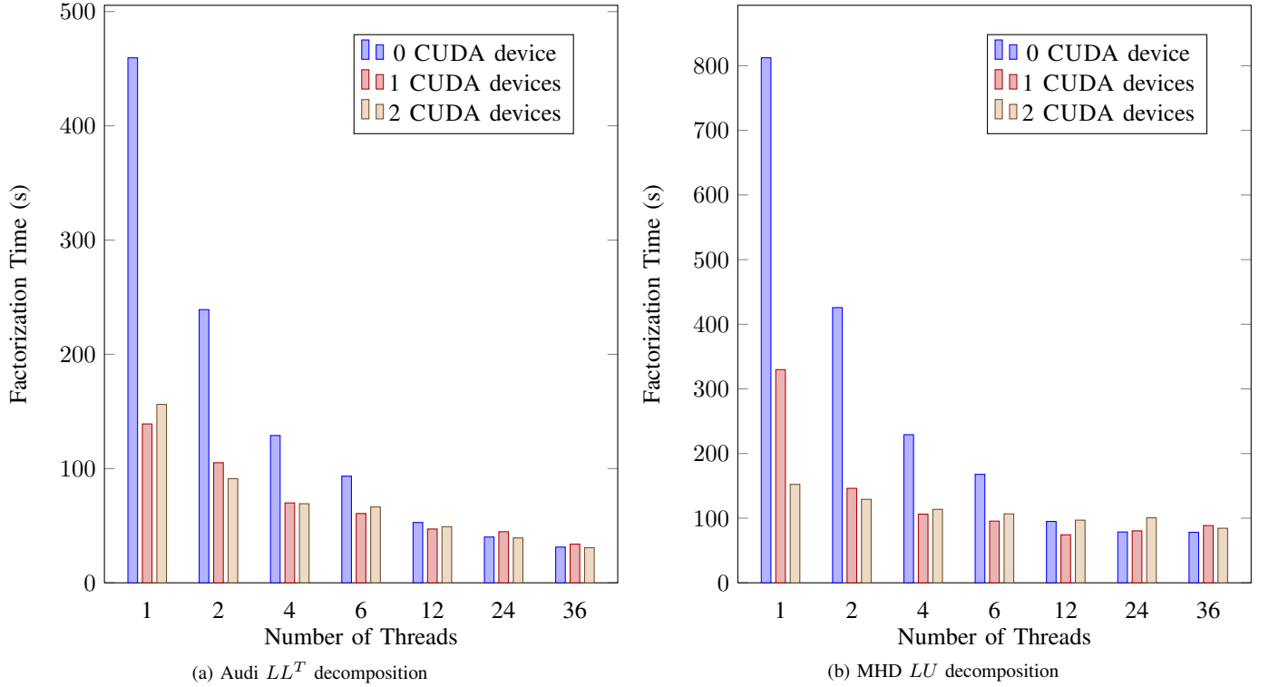
FIGURE 8: GPU results on Romulus (single precision)
