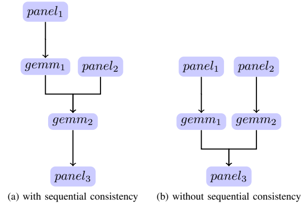
FIGURE 4: Task graph
