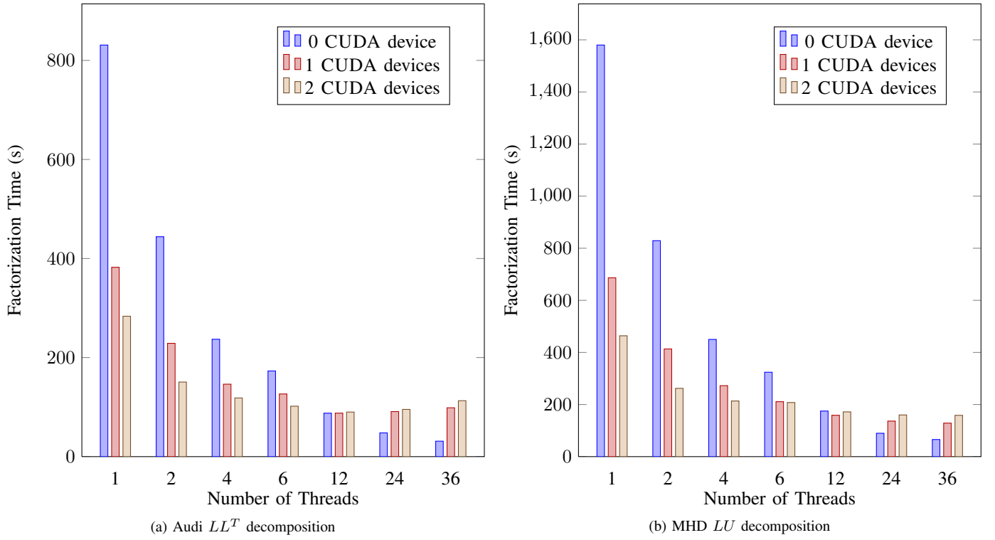
FIGURE 9: GPU results on Romulus (double precision)
