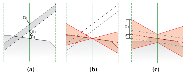
Figure 7: Ray refinement for transient edges. (a) A thin object intersection near the boundary of a pixel, which could be totally missed by ray intersection points. (b) Uncertainty region for the third intersection point and approximation planes for the other two points. Intersections between the uncertainty region and the approximation planes indicate the existence of transient edges. (c) Surface uncertainty region with a narrow face.
