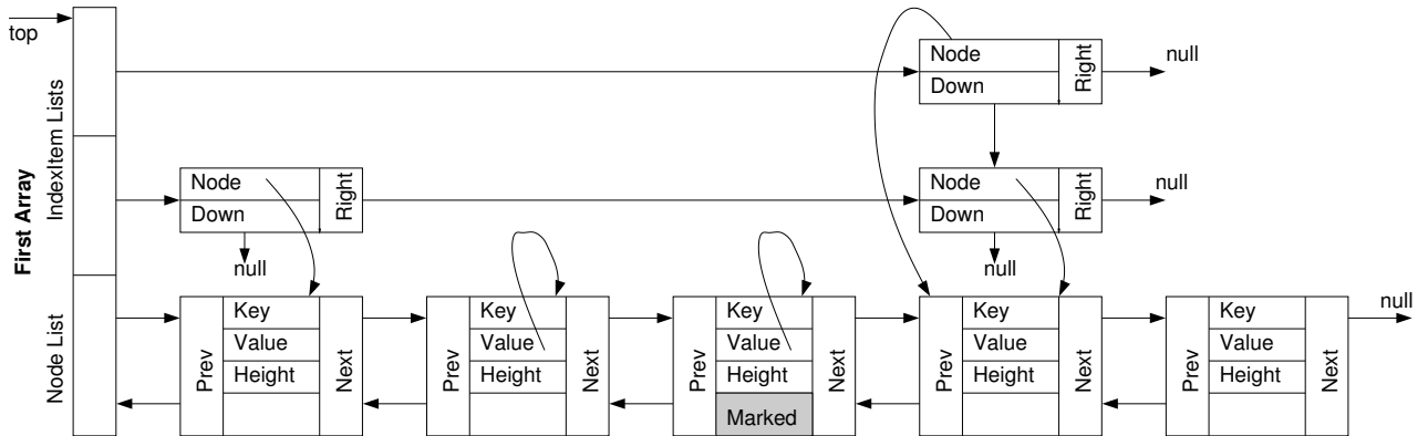
Figure 2: Skip list structure
