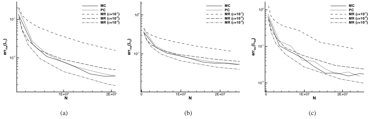
Figure 27: Error norms of the mean of the variable y_2 for the 1D Kraichnan-Orszag (for long time T = 500 ) problem with uniform pdf in the L_1 (a), L_2 (b) and L_\infty (c) spaces.
