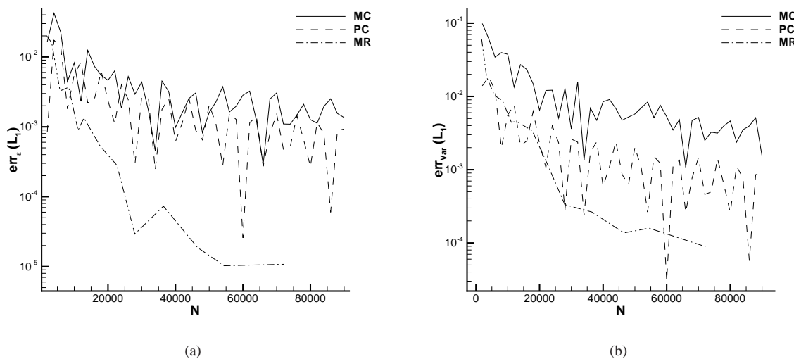
Figure 10: Errors for the mean (a) and variance (b) in the L_1 norm for the equation (29) with m_L = 1 and \varepsilon = 10^{-2} .
