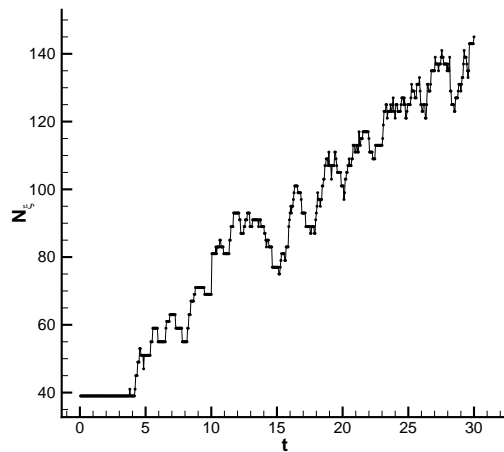
Figure 38: Evolution of the number of points in time for the TE algorithm with \epsilon = 10^{-1} , m_L = 4 and m_{\max} = 8 , 1D Kraichnan-Orszag problem with discontinuous unsteady pdf.
