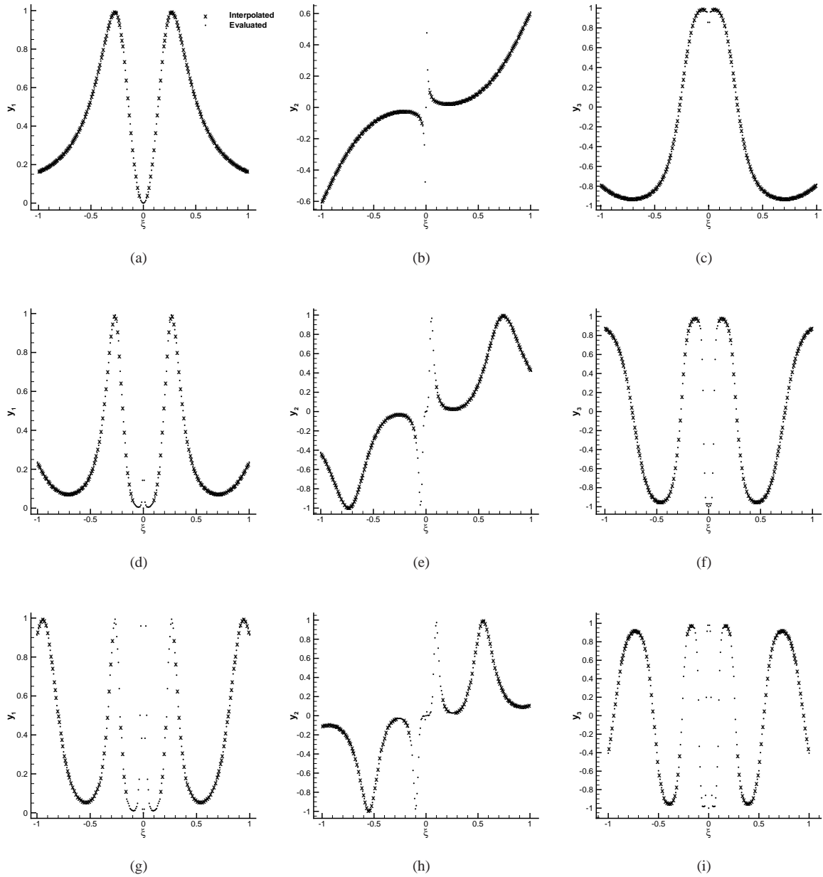
Figure 17: Time evolution of the variables y_1 (left), y_2 (middle) and y_3 (right) at different time steps: t = 10 ((a), (b) and (c)), t = 20 ((d), (e) and (f)) and t = 30 ((g), (h) and (i)). x interpolated points and \cdot evaluated ones.
