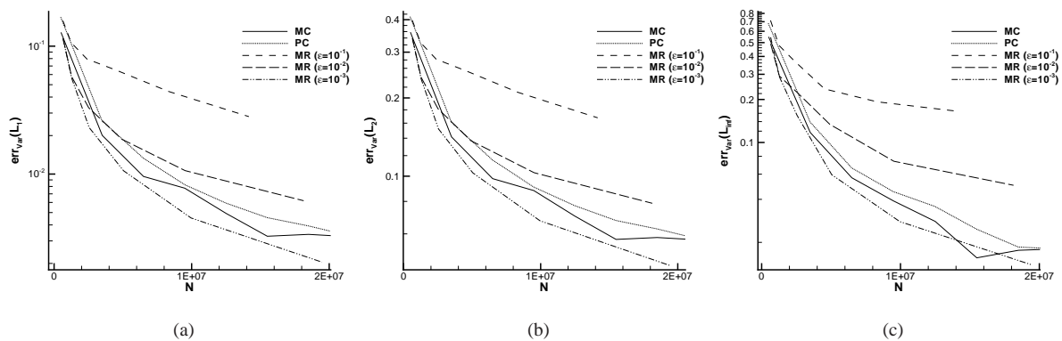
Figure 26: Error norms of the variance of the variable y_1 for the 1D Kraichnan-Orszag (for long time T = 500 ) problem with uniform pdf in the L_1 (a), L_2 (b) and L_\infty (c) spaces.
