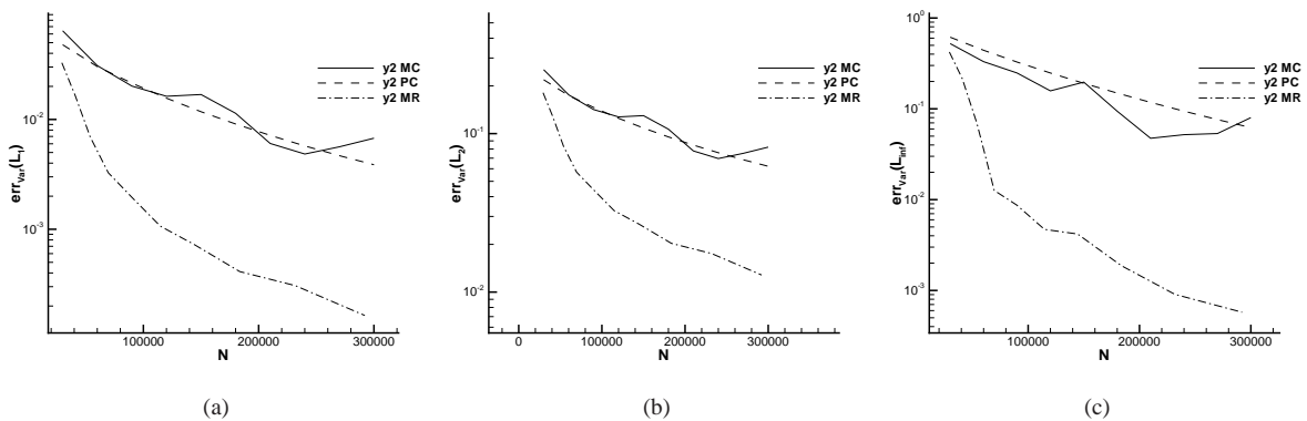
Figure 21: Error norms of the mean of the variable y_2 for the 1D Kraichnan-Orszag problem with uniform pdf in the L_1 (a), L_2 (b) and L_\infty (c) spaces.
