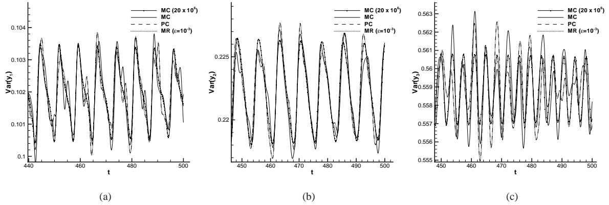
Figure 24: Comparison of the time evolution for the variance of the variables y_1 (a), y_2 (b) and y_3 (c) in the Kraichnan-Orszag problem with uniform distribution ( T = 500 ). The last time steps are computed with the Monte Carlo, Polynomial Chaos and TE algorithm, \varepsilon = 10^{-3} , m_L = 4 and m_{\max} = 12 ( N_\varepsilon = 3760 ), and compared to the Monte Carlo reference solution N_\varepsilon = 20 \times 10^6 .
