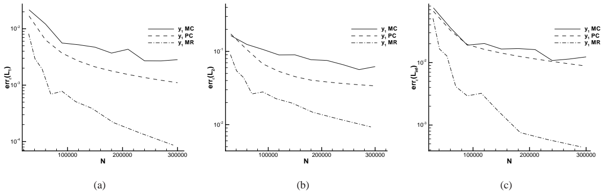
Figure 19: Error norms of the mean of the variable y_1 for the 1D Kraichnan-Orszag problem with uniform pdf in the L_1 (a), L_2 (b) and L_\infty (c) spaces.
