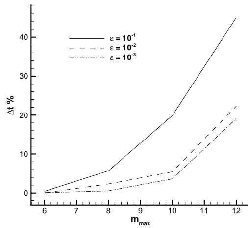
Figure 31: Time saved using the TE algorithm on the Kraichnan-Orszag problem with different threshold and different maximal levels. The coarsest level is equal to m_L = 4 for all the computations.
