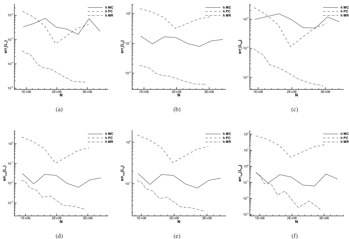
Figure 41: Error norms of the mean (top) and variance (bottom) of the variable h of the aeroelastic problem in the L_1 ((a) and (d)), L_2 ((b) and (e)) and L_\infty ((c) and (f)) spaces.
