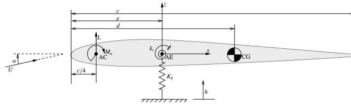
Figure 39: Sketch of the wing section aeroelastic problem with the forces and the convention adopted.
