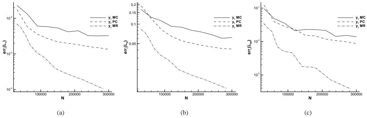
Figure 34: Error norms of the mean of the variable y_1 for the 1D Kraichnan-Orszag with unsteady pdf problem in the L_1 (a), L_2 (b) and L_\infty (c) spaces.
