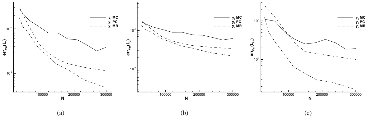
Figure 20: Error norms of the variance of the variable y_1 for the 1D Kraichnan-Orszag problem with uniform pdf in the L_1 (a), L_2 (b) and L_\infty (c) spaces.
