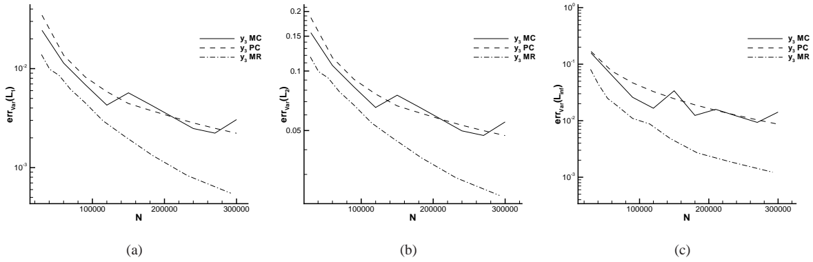
Figure 22: Error norms of the mean of the variable y_1 for the 1D Kraichnan-Orszag problem with uniform pdf in the L_1 (a), L_2 (b) and L_\infty (c) spaces.
