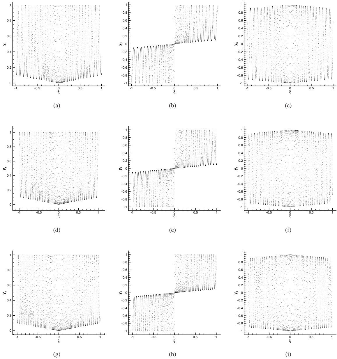
Figure 29: Time evolution of the variables y_1 (left), y_2 (middle) and y_3 (right) at different time steps: t = 300 ((a), (b) and (c)), t = 400 ((d), (e) and (f)) and t = 500 ((g), (h) and (i)).
