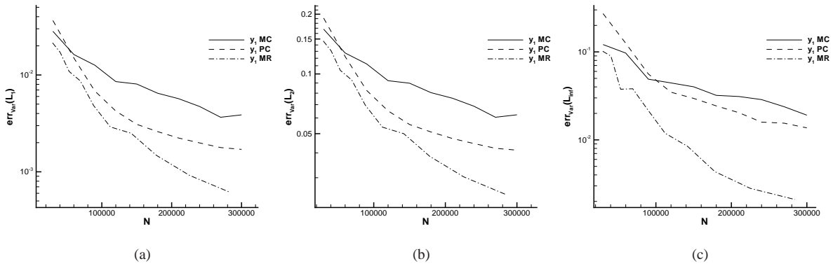
Figure 35: Error norms of the variance of the variable y_1 for the 1D Kraichnan-Orszag problem with unsteady pdf in the L_1 (a), L_2 (b) and L_\infty (c) spaces.
