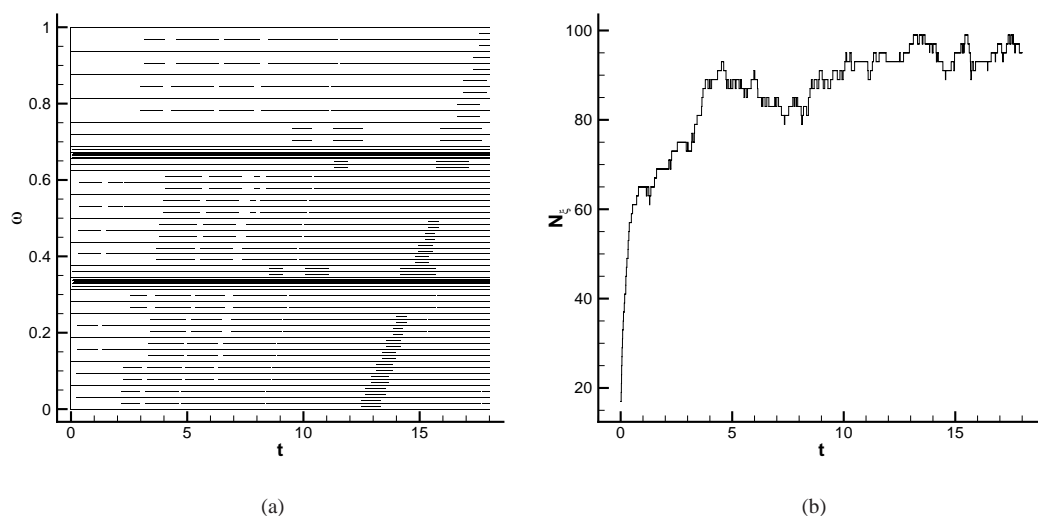
Figure 43: Patterns of the evaluations in the space t - \omega ((a)) and the number of points in the stochastic space N_g employed by the TE algorithm with m_{\max} = 16 (b)).
