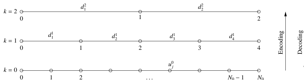
Figure 1: Harten's multiresolution classical notation.
