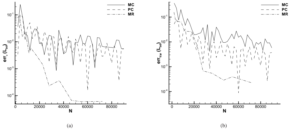
Figure 12: Errors for the mean (a) and variance (b) in the L_\infty norm for the equation (29) with m_L = 1 and \varepsilon = 10^{-2} .
