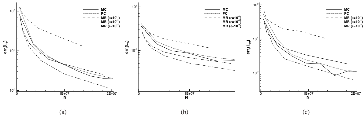
Figure 25: Error norms for the mean of the variable y_1 of the 1D Kraichnan-Orszag (for long time T = 500 ) problem with uniform pdf in the L_1 (a), L_2 (b) and L_\infty (c) spaces.
