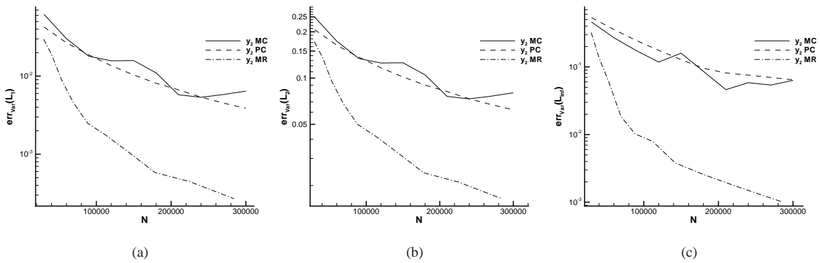
Figure 36: Error norms of the variance of the variable y_2 for the 1D Kraichnan-Orszag problem with unsteady pdf in the L_1 (a), L_2 (b) and L_\infty (c) spaces.
