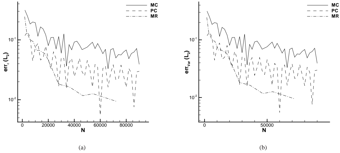
Figure 11: Errors for the mean (a) and variance (b) in the L_2 norm for the equation (29) with m_L = 1 and \varepsilon = 10^{-2} .
