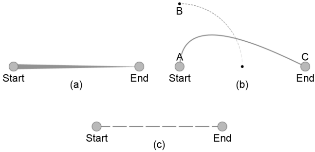
Figure 2: The directed-edge representations that were evaluated: (a) tapered from wide (start) to narrow (end), (b) biased clockwise curvature from high (start) to low (end) curvature, and (c) animated, in which a pattern moves from start to end along a straight line.
