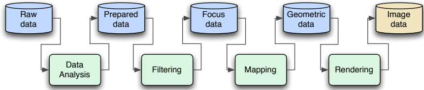
Figure 6.2: The Visualisation Pipeline, adapted from Dos Saltos and Brodlić [5]
