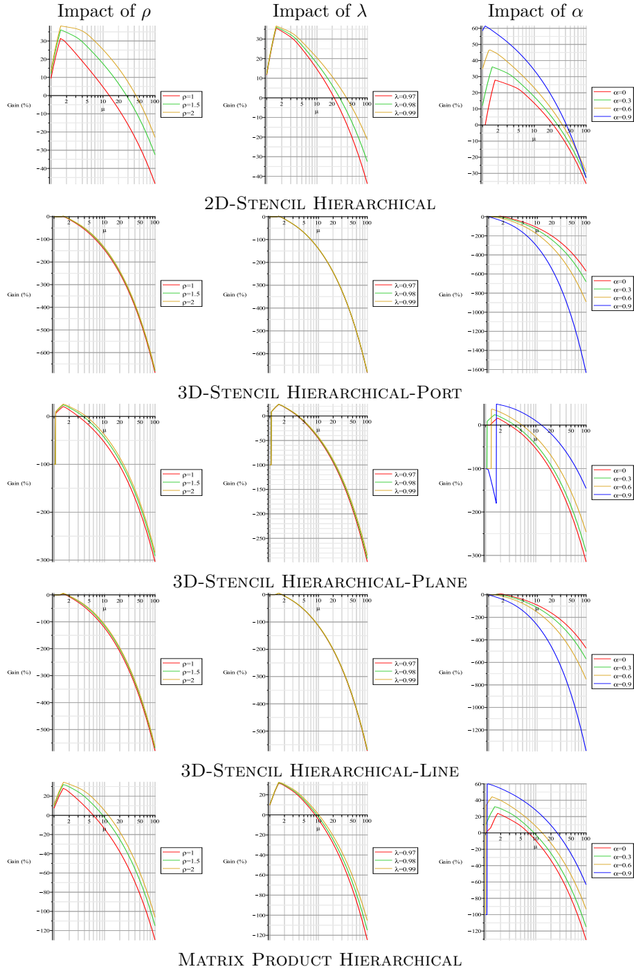
Figure 10: Impact of the parameters \rho , \lambda , and \alpha on the relative gain of the hierarchical protocols with respect to the coordinated one on the K-computer platform.
