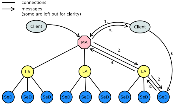
Figure 3: DIET architecture
