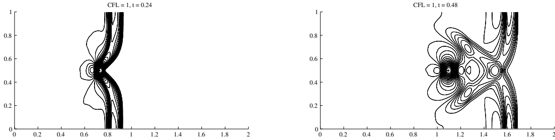
Figure 4: Perturbation to the lake at rest when solved with the discontinuous STB scheme with \text{CFL} = 1 . 50 water-height contours between values 0.992 and 1.012 at t = 0.24 (left) and t = 0.48 (right) are plotted.
