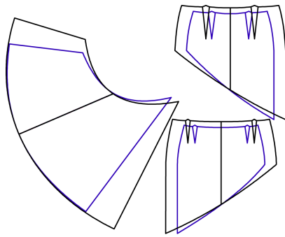
Figure 2: Traditional patterns for a skirt for small and large sizes (©www.osinka.ru).
