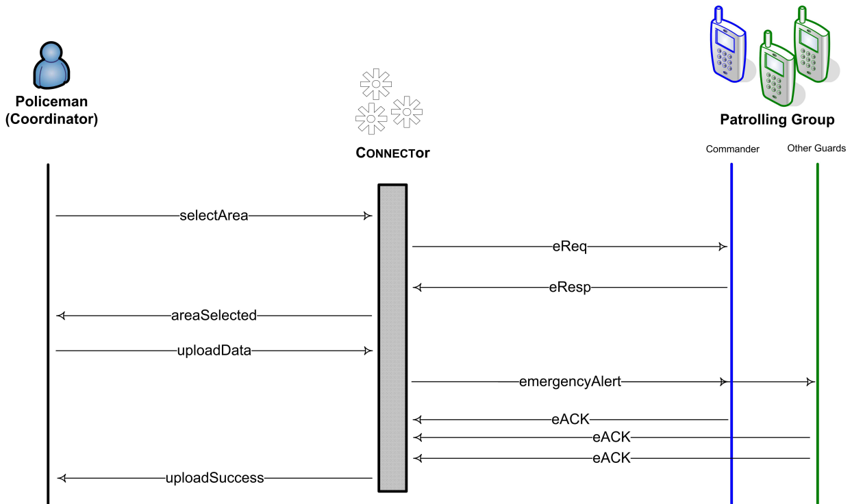
Figure 3.18: Terrorist Alert Scenario: Sequence Diagram of the Messages Exchange
