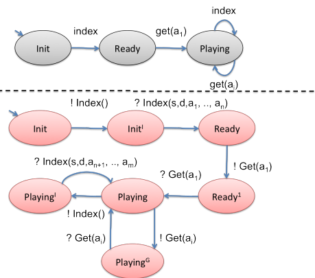
Figure 5.16: Simplified LTS describing the behaviour of an HLS Client
