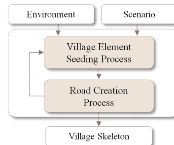
Fig. 3 Algorithm for the village skeleton growth.
