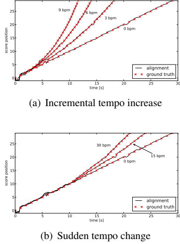
Fig. 2. Alignment to a synthetic track.
