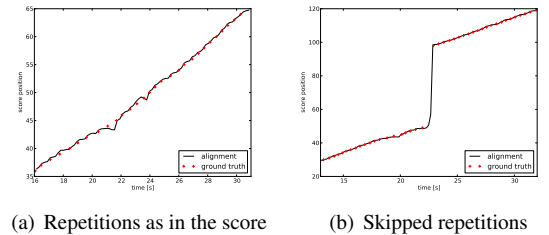
Fig. 3. Alignment of a performance with optional repetitions.
