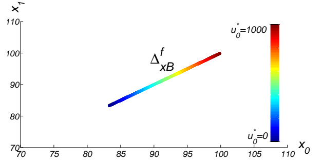
Fig. 5. Numerical example for the set \Delta_{xB}^f (color line). The left end of the line corresponds to the input flow vector: u_0^* = 0 , u_1^* = 0 while the right one is for u_0^* = 1000 , u_1^* = 0 .
