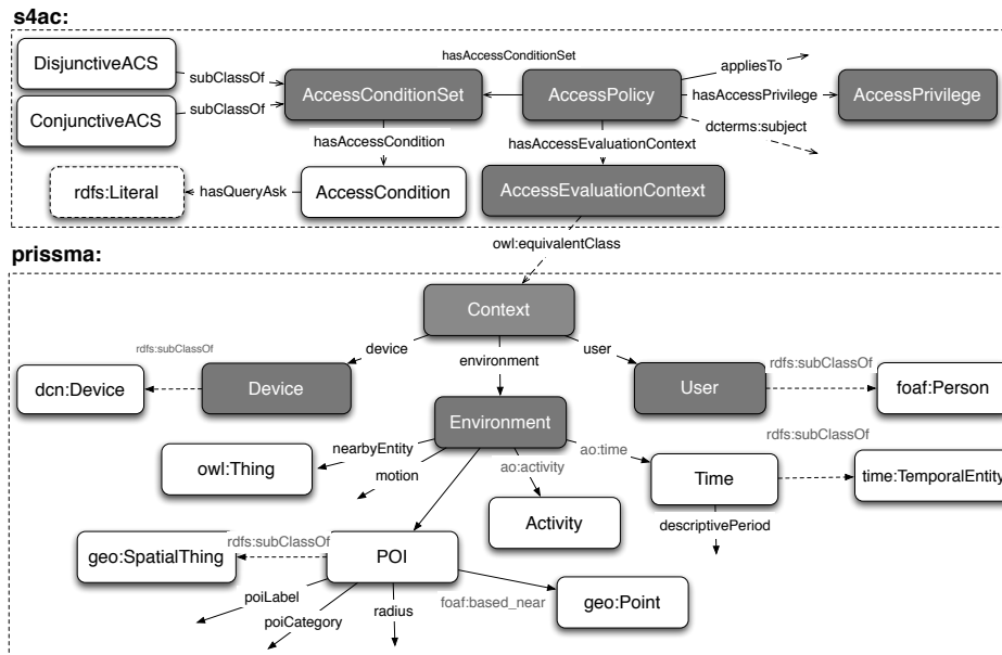
Figure 1: The model at a glance (grey boxes represent core classes).
