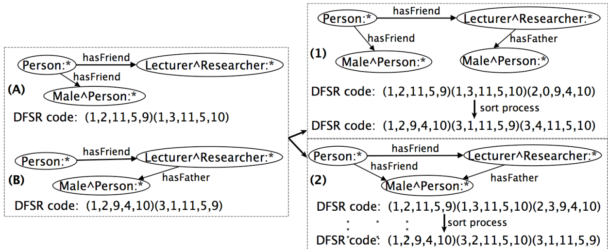
Figure 9. Join two IRDF graph patterns when the two unlinked nodes of the specific IRDF triples are identical.
