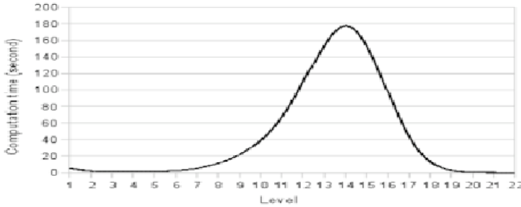
Figure 14. Computation time per level.
