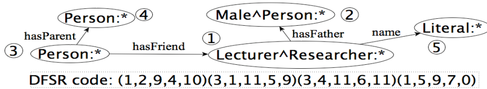
Figure 4. IRDF Graph pattern and its minimum DFSR code.
