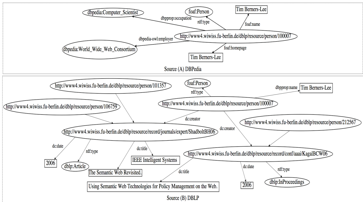
Figure 1. RDF graphs from of DBpedia and DBLP dataset.
