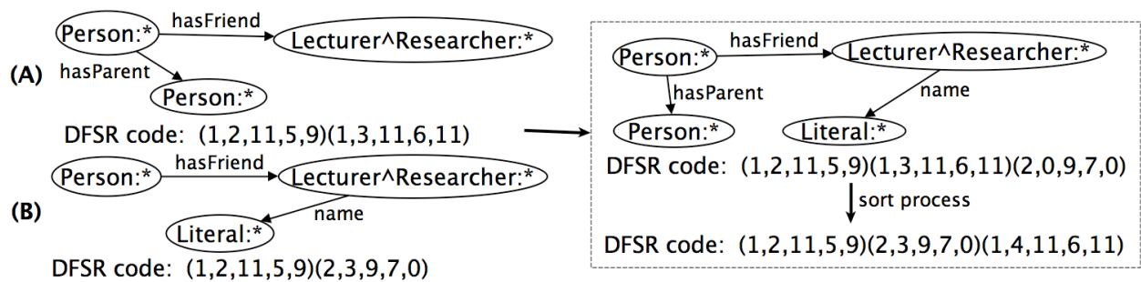
Figure 8. Join two IRDF graph patterns, when the two unlinked nodes of the specific IRDF triples are different.
