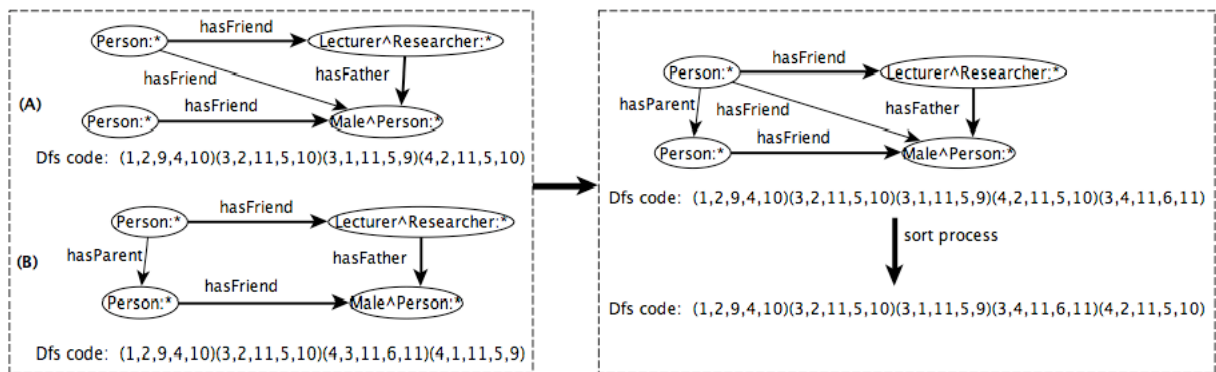
Figure 11. Join two IRDF graph patterns with the two specific IRDF triples linked to kernel by two nodes.
