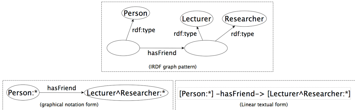
Figure 3. Graphical notation form and linear textual form.
