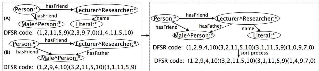
Figure 10. Join two IRDF graph patterns with one of specific IRDF triples linked to kernel by two nodes.
