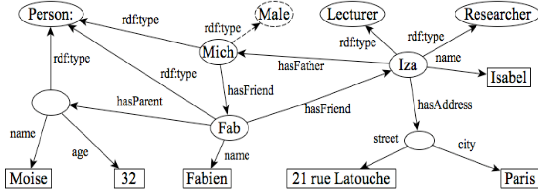
Figure 2. Example of RDF store.
