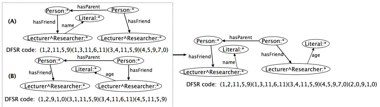
Figure 7. Example of joining two IRDF graph patterns of size 4, case 2.
