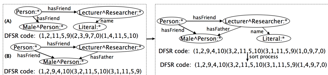
Figure 10: Join two graph patterns with one of specific edges linked to kernel by two nodes.
