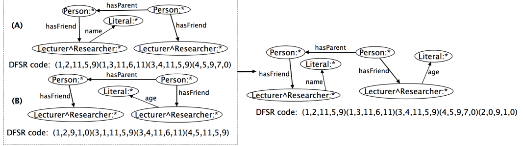
Figure 7: Example of joining two DFSR codes of size 4, case 2.
