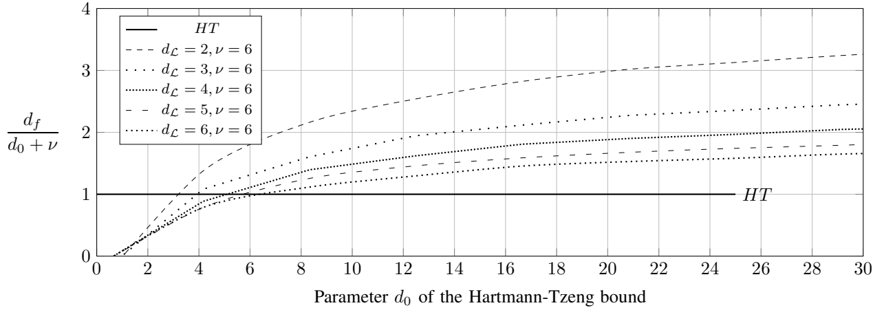
Fig. 2. Illustration of the fraction d_f/(d_0 + \nu) of our bound d_f of (11) to the Hartmann–Tzeng bound d_0 + \nu for \nu = 6 , d_0 = 2, \dots, 30 , c_1 = c and c_2 = 1 . We used an RS code as non-zero-locator code with distance d_{\mathcal{L}} = c - \nu (see Table II).
