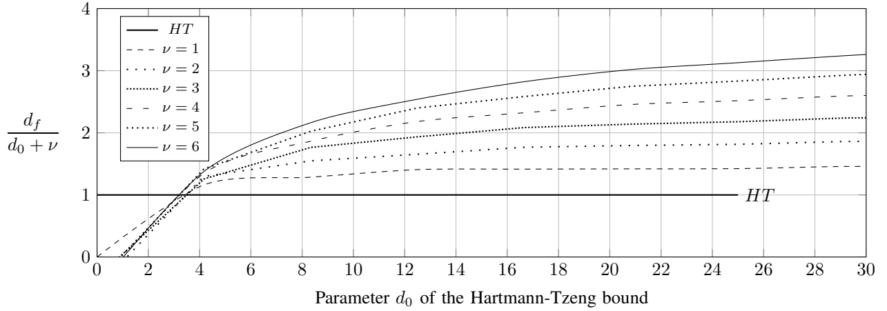
Fig. 1. Illustration of the fraction d_f/(d_0 + \nu) of our bound d_f of (11) to the Hartmann–Tzeng bound d_0 + \nu for \nu = 1, \dots, 6 and d_0 = 2, \dots, 30 . The parameters of the HT bound are c_1 = \nu + 2 and c_2 = 1 (see Table III). We used a single parity check code as non-zero-locator code. Our bound d_f is for d_0 > 3 better than the HT bound.
