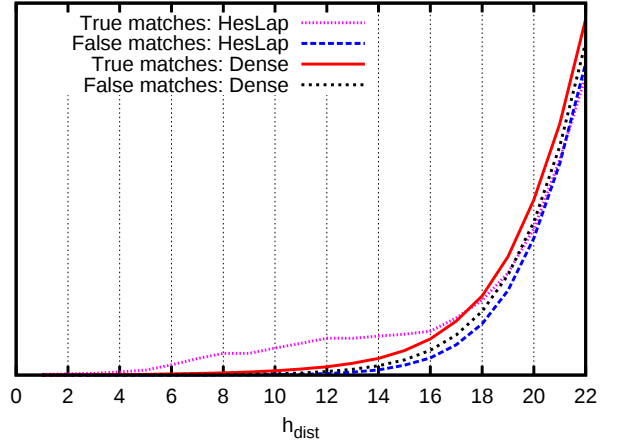
Figure 3: Empirical distribution of true matches and false matches as a function of the Hamming distance ( h_{\text{dist}} ). We only show a zoomed version for h_{\text{dist}} = 0 to 22. Measurements are performed on PASCAL VOC 2007 dataset (category boat ).
