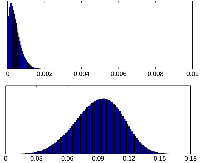
Figure 4: Distribution of similarity scores (a) before and (b) after power normalization (with \alpha = 0.3 ). Note the change in the scales. The scores are obtained for trainval set of PASCAL VOC 2007 dataset.
