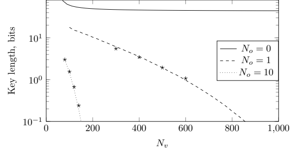
Fig. 5. key length per symbol for SS: DWR = 10dB , \epsilon = 10^{-2} , * represents Monte-Carlo simulations using 10^3 random keys and observing 10^2 times N_o contents.
