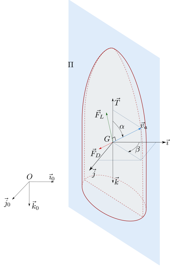
Fig. 2. Aerodynamic forces and (\alpha, \beta) angles.
