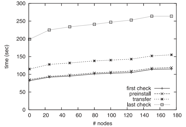
Fig. 4 Time (in seconds) to deploy and boot a new OS on a cluster with Kadeploy2.
