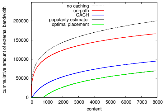
Figure 1: Median of the aggregate traffic on peer-links, ordered by popularity
