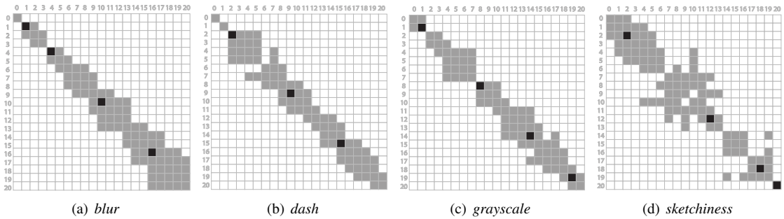
Figure 11: Black squares show our chosen representative levels, and gray ones indicate levels that are not significantly different.
