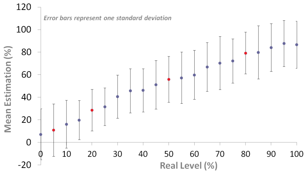
Figure 7: Real vs. estimated blur with red dots for distinct levels.
