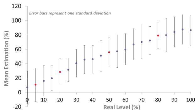
Fig. 7. Real vs. estimated blur with red dots for distinct levels.
