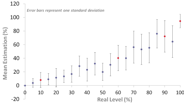
Fig. 10. Real vs. estimated sketchiness with red dots for distinct levels.
