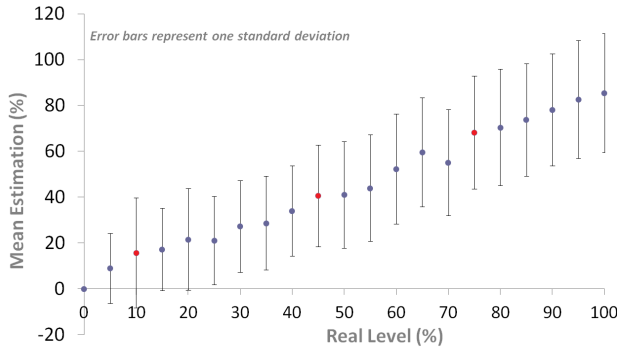
Fig. 9. Real vs. estimated dashing with red dots for distinct levels.
