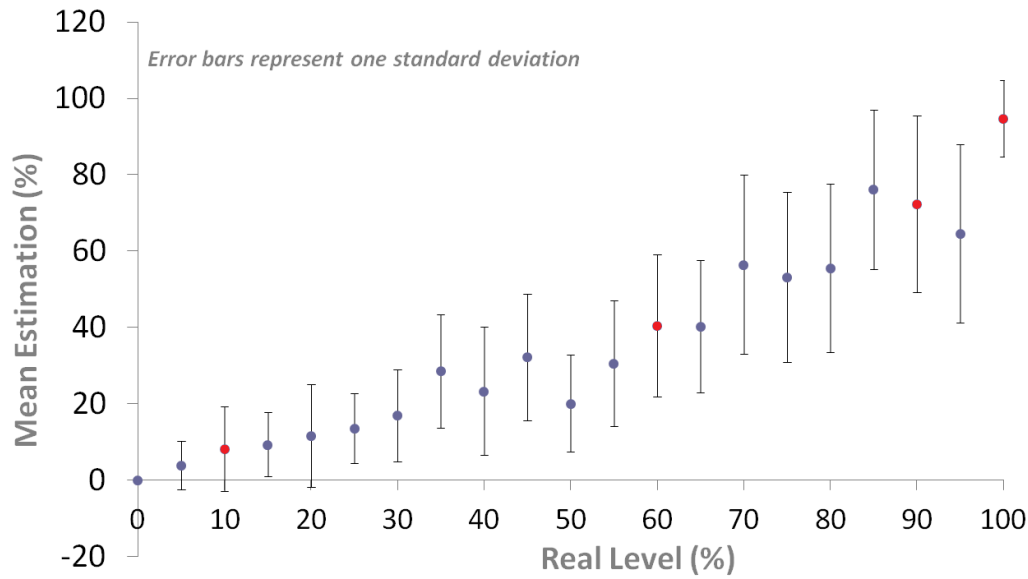
Figure 10: Real vs. estimated sketchiness with red dots for distinct levels.
