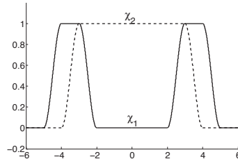
Figure 3: Truncation functions
