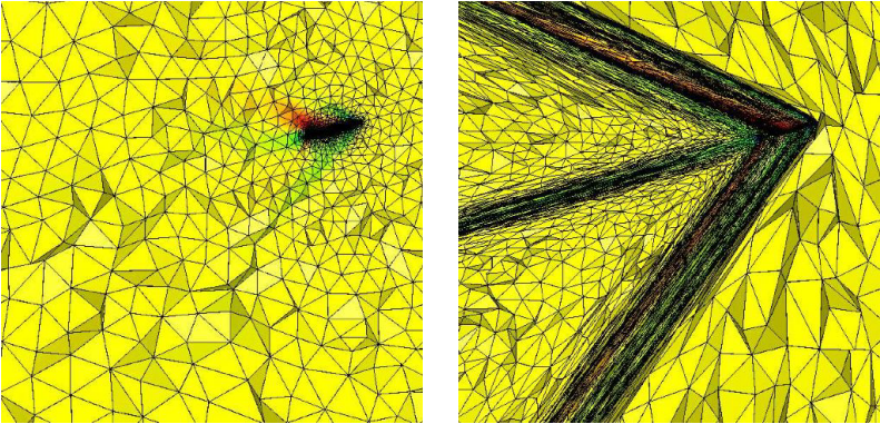
Figure 4: Supersonic flow around an airplane (mach 1.6, angle attack 3 degree, diameter of the box 1km): volumic cut on initial and adapted meshes.
