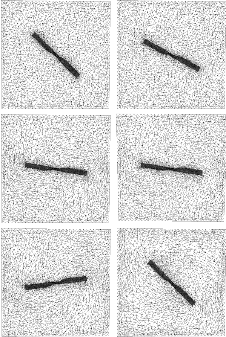
Figure 8: Propeller in rotation: cut through the tetrahedra after 1, 45, 99, 100, 145 and 500 rotations.
