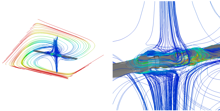
Figure 9: Propeller in rotation: streamlines.
