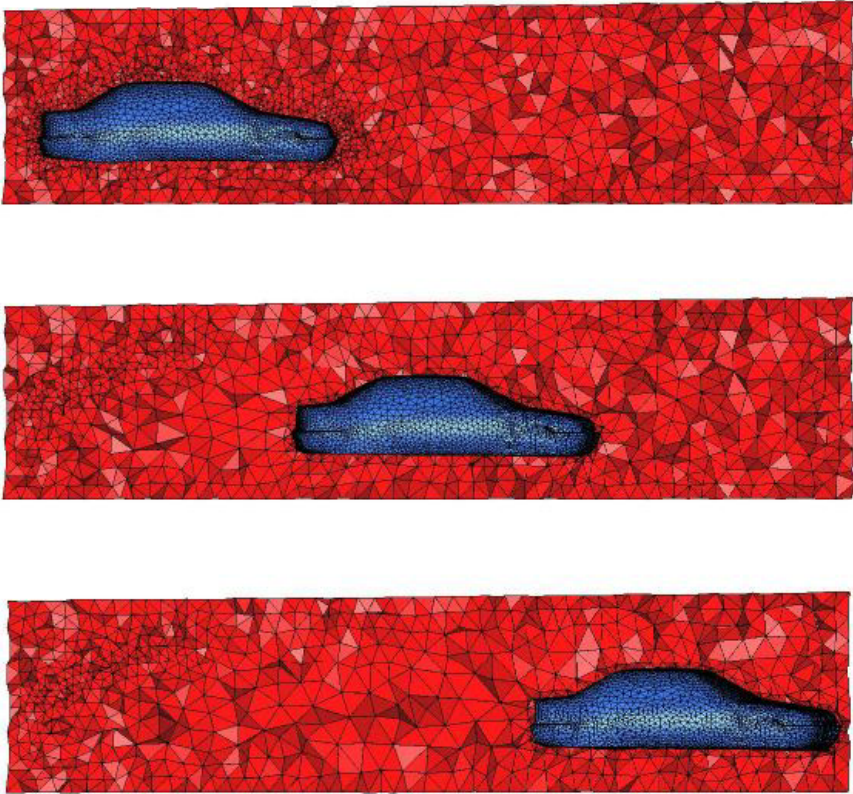
Figure 6: Volumic cuts after one, 75 and 150 boundary moves.
