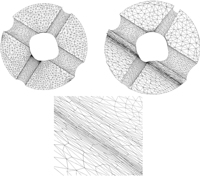
Figure 3: Volumic cuts on initial mesh and adapted mesh. Zoom on anisotropic meshes.
