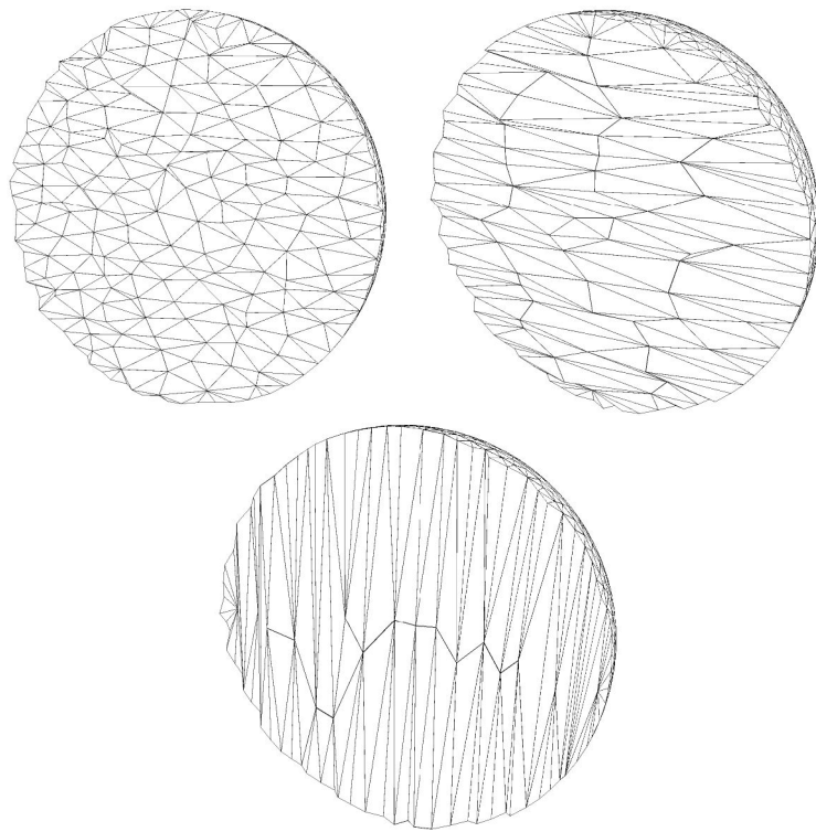
Figure 2: Volumic cut in adapted meshes: in the left top \alpha = 2 , \beta = 1 et \gamma = 1 ; in the right top \alpha = 1 , \beta = 5 et \gamma = 1 ; on the bottom \alpha = 1 , \beta = 1 et \gamma = 10 .
