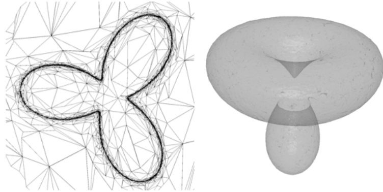
Figure 5: Example of mesh adaptation to capture an implicitly defined surface: cutting plane through tetrahedral element (left) and isosurface reconstruction (right)
