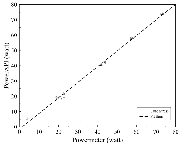
Figure 3. The accuracy of POWERAPI when stressing the processor cores.
