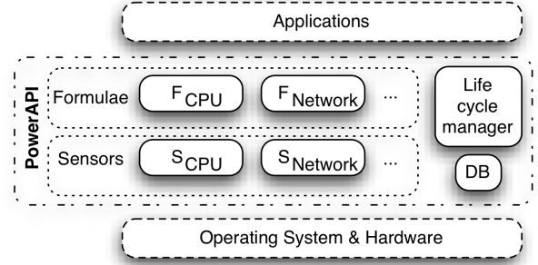
Figure 1. POWERAPI Reference Architecture.
