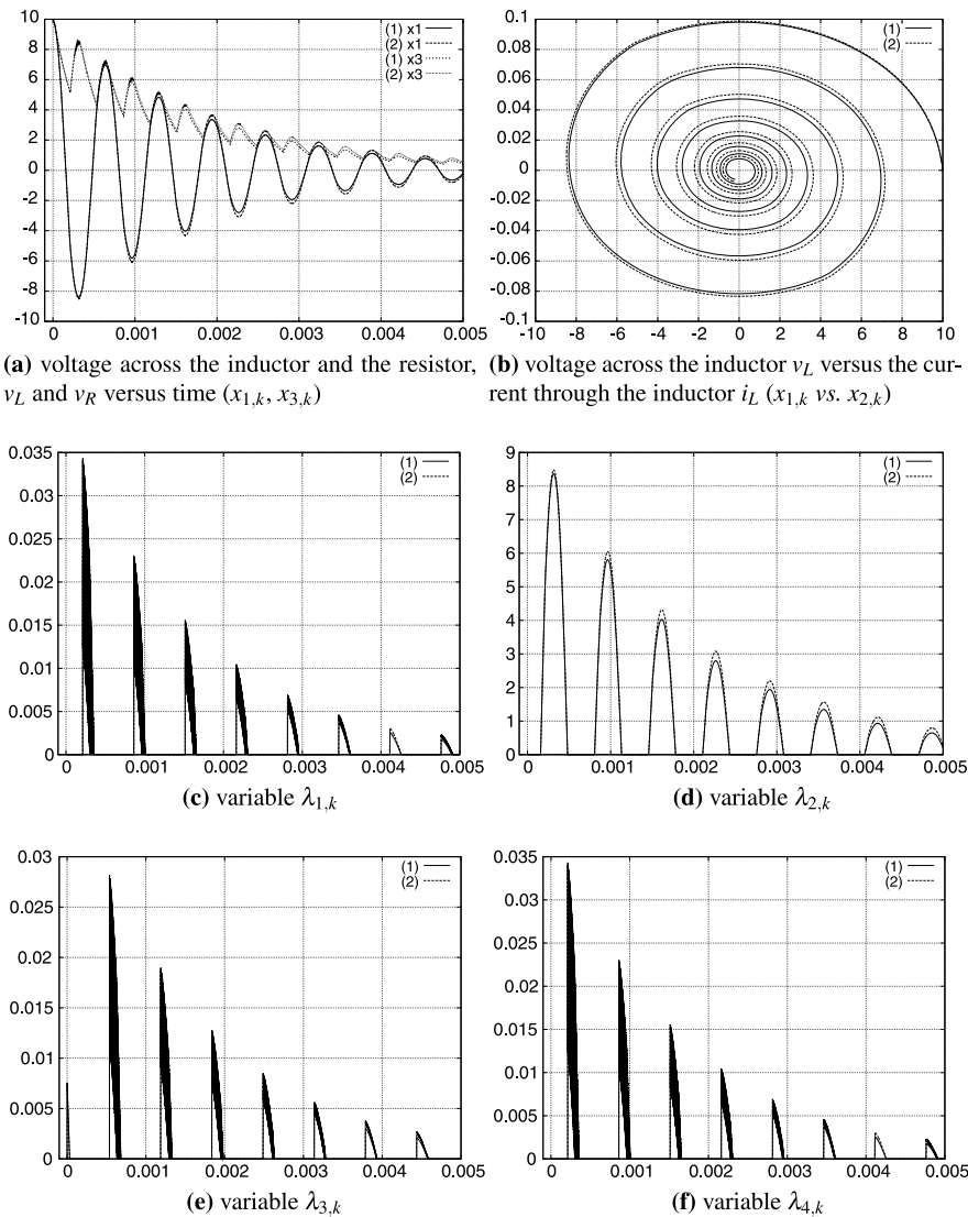
Fig. 14.7 Simulation of the configuration in Fig. 14.5 with the scheme (14.25) for two values of parameters: (1) \theta = 1, \gamma = 1 ; (2) \theta = 1/2, \gamma = 1/2 . Some instabilities are generated for the approximation of the BV functions
