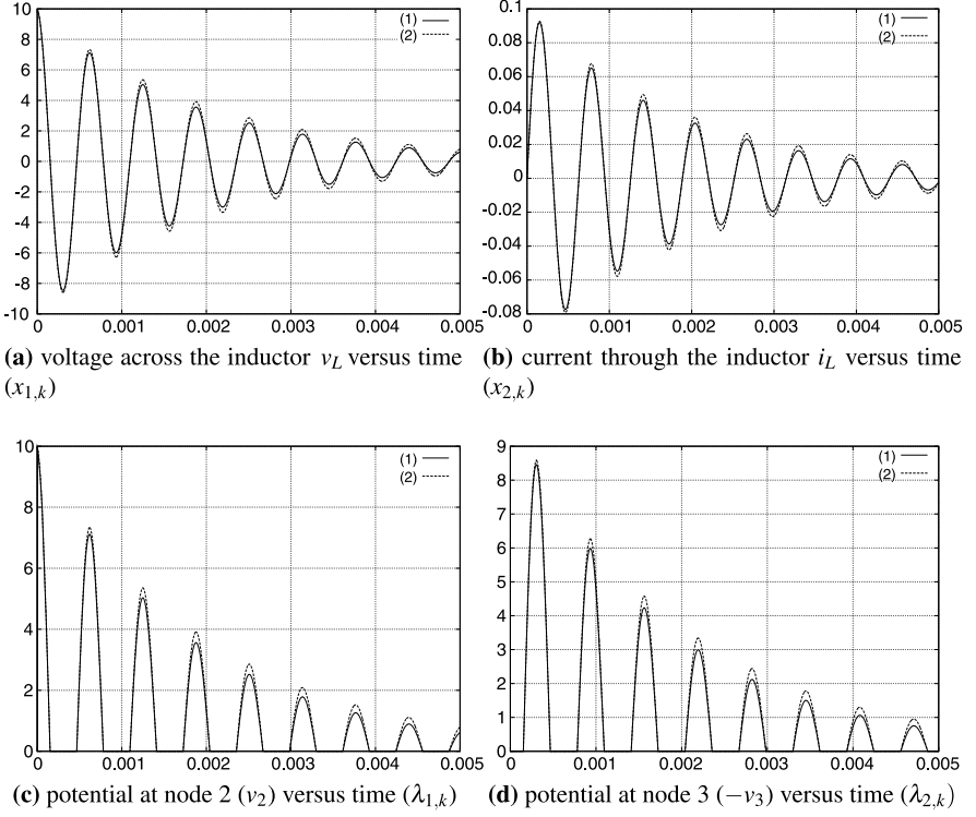
Fig. 14.3 Simulation of the circuit on Fig. 14.2 with the scheme (14.25) for two values of parameters: (1) \theta = 1 , \gamma = 1 ; (2) \theta = 1/2 , \gamma = 1/2
