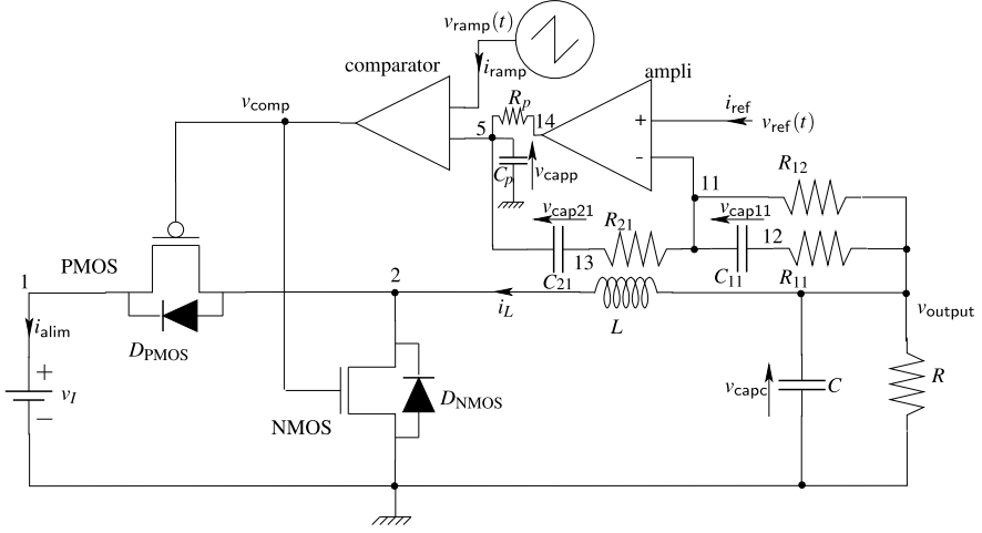
Fig. 14.9 Buck converter
