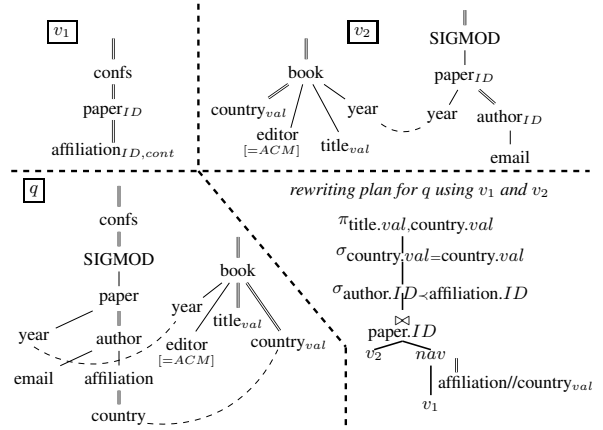
Figure 3: Pattern query and views, and algebraic rewriting.
