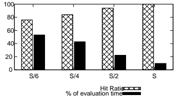
Figure 8: ROA performance on the workload Q_4 .
