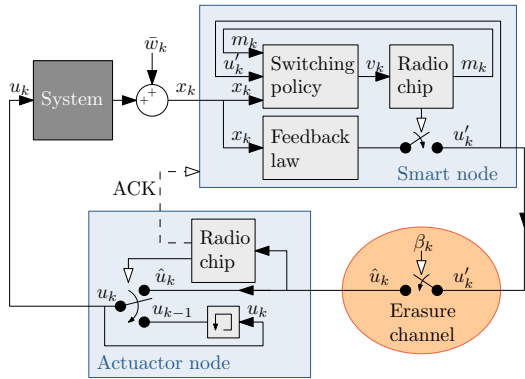
Fig. 1. Block diagram of the problem setup. The smart node measures the noisy state x_k from the system, it computes the feedback law u'_k and decides whether to send it or not to the actuator node. \hat{u}_k is equal to u'_k when a transmission occurs, or to \emptyset otherwise. The receiver is then able to determine if it has received an update or not. \beta_k equals 1 when the transmission is successful or 0 when there is a dropout.
