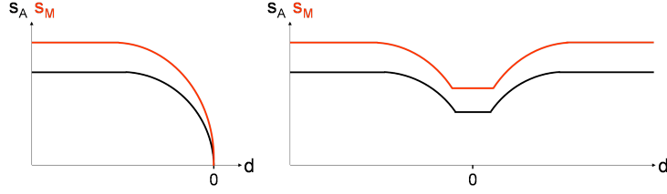
Figure 3: Example average ( s_A ) and maximum ( s_M ) speed profiles generated a pair ( M_t^n = m_i, I_t^n = 1 ) (left) and ( M_t^n = m_i, I_t^n = 0 ) (right). When I_t^n = 0 , the lowest speed in the profile is a function of the curvature of the path associated with the maneuver m_i .
