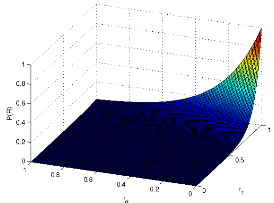
Fig. 2. Probability density function P(R_U) .
