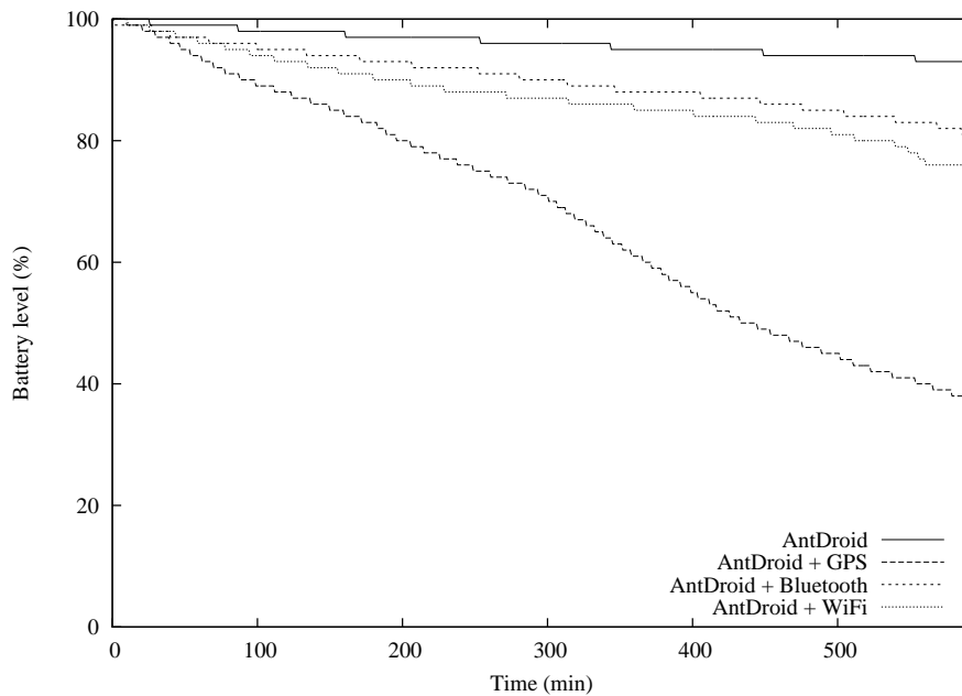
Figure 6: Impact of ANTDRROID on the battery lifespan.
