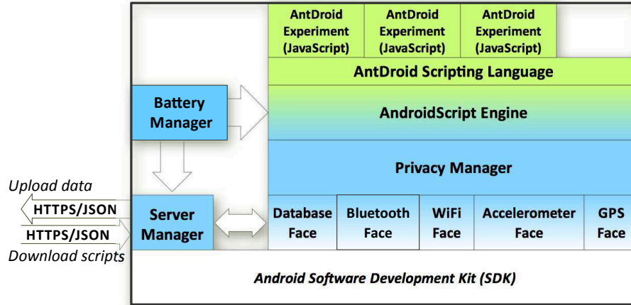
Figure 2: Architecture of the ANTDRROID Software Architecture
