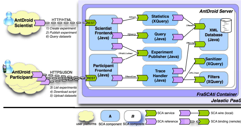
Figure 1: Architecture of the ANTDRROID Software Platform.
