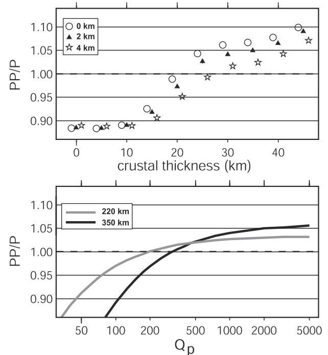
Figure 2. (a) Predictions of PP/P amplitude ratios for models with the same seismic velocity, density, and Q structure as in PREM, but in which the thickness of the crust is varied between 0 and 50 km and the ocean has a water depth of 0 km (circle), 2 km (triangle), or 4 km (star). The effect of an ocean on PP/P is large only when the crust is thicker than 15 km. These models are irrelevant since oceanic crust is typically thinner than 10 km. (b) Predictions of PP/P for models in which a constant value of Q_p in the uppermost 220 km (light grey line), or uppermost 350 km (dark grey line) of the mantle is varied. The velocity and density structures are the same as in PREM.
