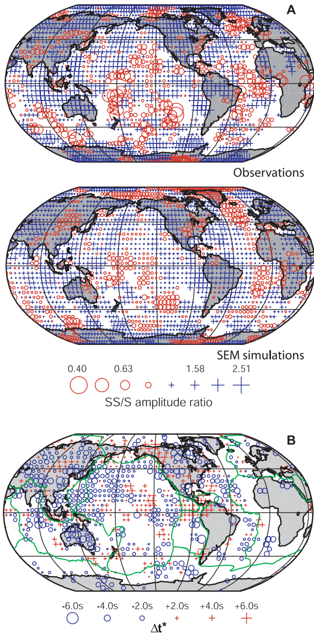
Figure 3. (a) Observed (top) and SEM predicted (bottom) SS/S amplitude ratios with respect to PREM and Harvard CMT source parameters plotted at SS surface reflection points. Red circles represent negative SS/S residuals with respect to PREM, while blue '+' symbols represent positive SS/S anomalies. (b) \Delta t^*_{SS-S} distribution from Reid et al. [2001]. SS waveforms associated with positive (negative) \Delta t^*_{SS-S} values are relatively broad (narrow) compared to SS waveforms simulated using the PREM model. The data in both (a) and (b) have been smoothed by averaging at least 3 residuals with SS reflection points that fall within a circular cap with a radius of 5^\circ . It is expected that negative (positive) SS/S residuals correlate with positive (negative) values of \Delta t^*_{SS-S} .
