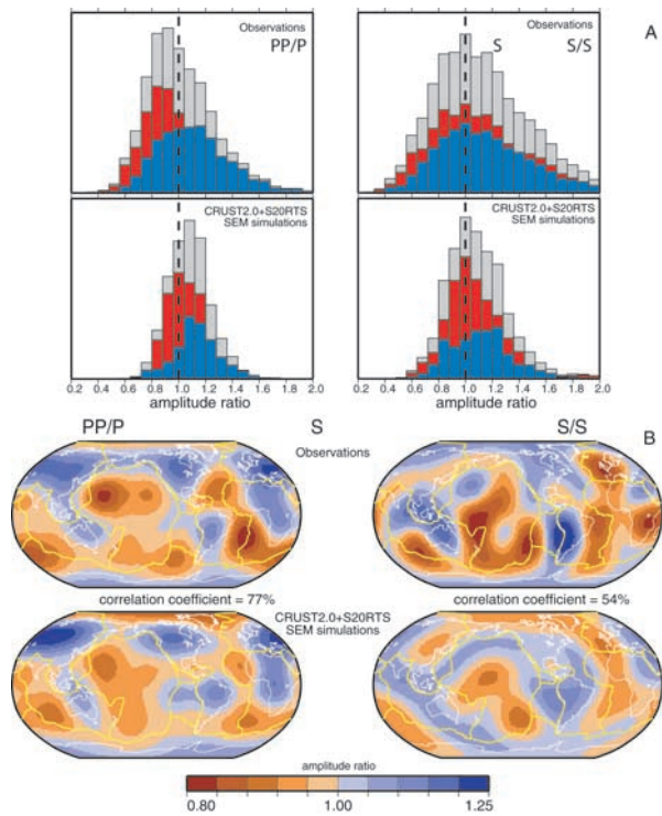
Figure 1. (a) Histograms of PP/P (left) and SS/S (right). The data are grouped according to whether the associated PP (or SS) surface reflection point is underneath the oceans (red) or continents (blue). (b) PP/P (left) and SS/S (right) amplitude ratios with respect to PREM and Harvard CMT source parameters, plotted at the PP surface reflection point. The top panel shows the observed amplitude ratios, while the lower panel shows amplitude ratios determined from the SEM synthetics. The large-scale trends in PP/P and SS/S are emphasized by expanding their values in spherical harmonics up to degree and order 6. The correlations between the observed and SEM predicted PP/P and SS/S maps are, respectively, 77% and 54%.
