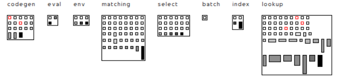
Fig. 6. Earliest x latest NOB
