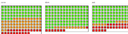
Fig. 10. Bug Lifetime
