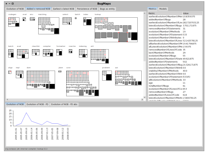
Fig. 2. BugMaps: history browser
